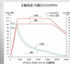
24,000 RPM 內藏式主軸 (選配)
