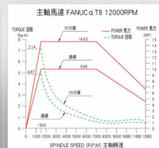
12,000 RPM 直結式主軸 (選配)
